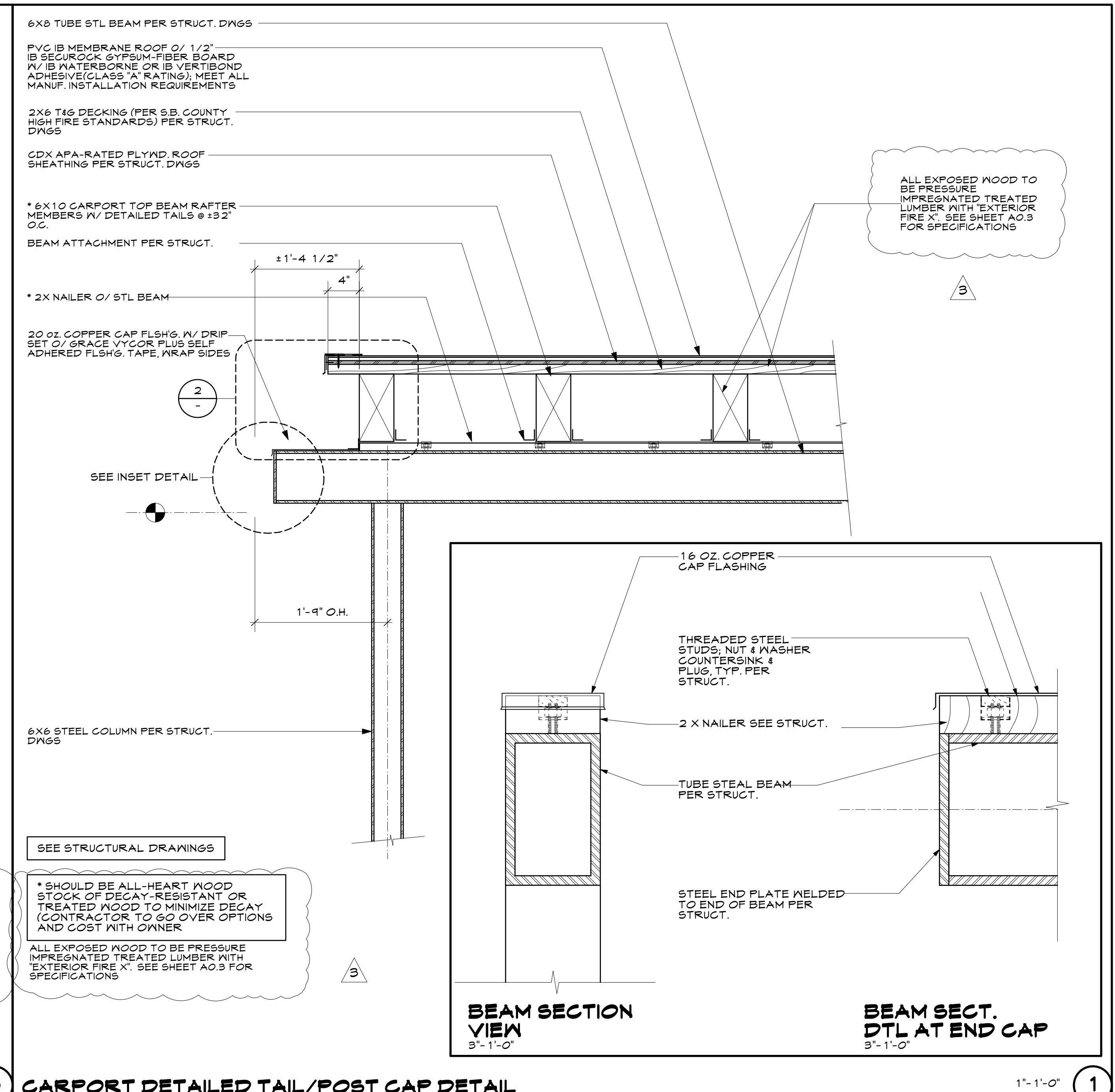
BEAM SECTION VIEW 3'-1'-0" 1
