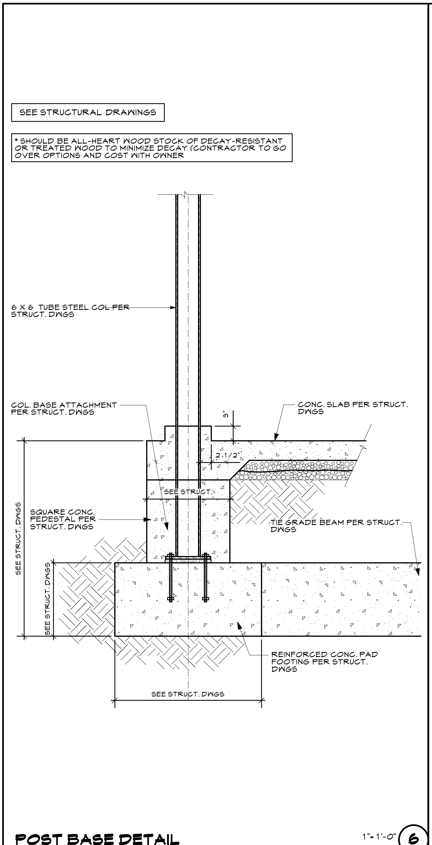
POST BASE DETAIL 1'-1'-0" 6
