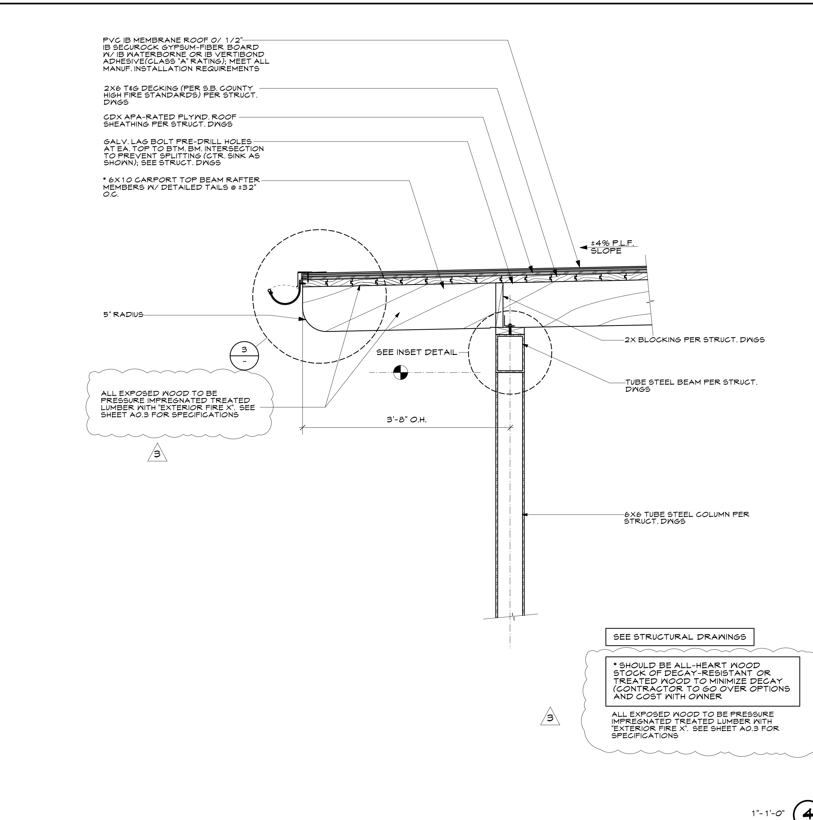
CARPORIT DETAILED TAIL/POST CAP DETAIL 1'-1'-0" 4
